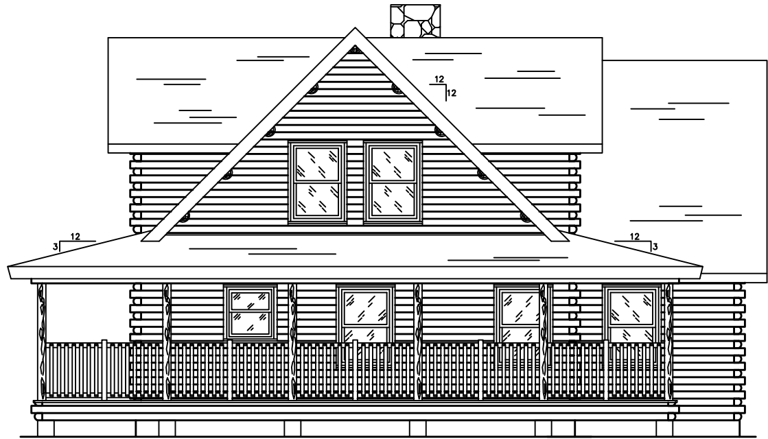
ELEVATION D
