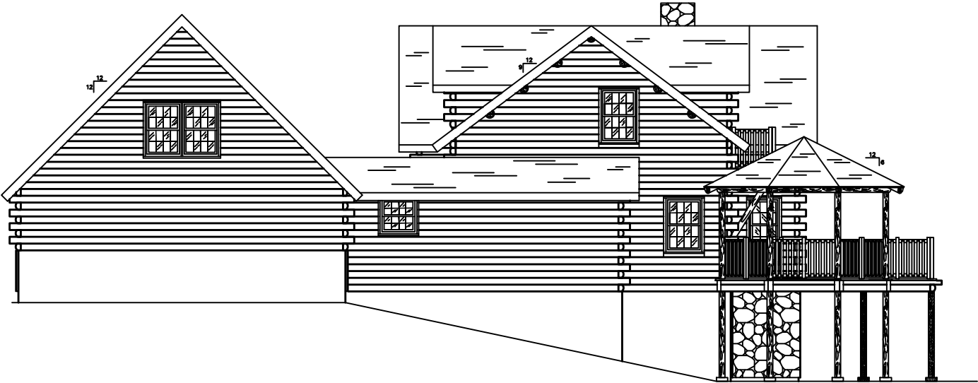
ELEVATION D
