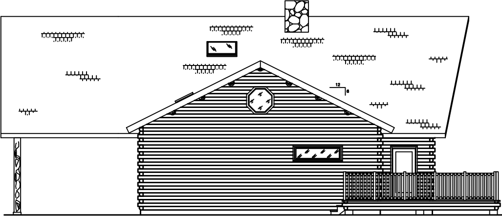
ELEVATION D
