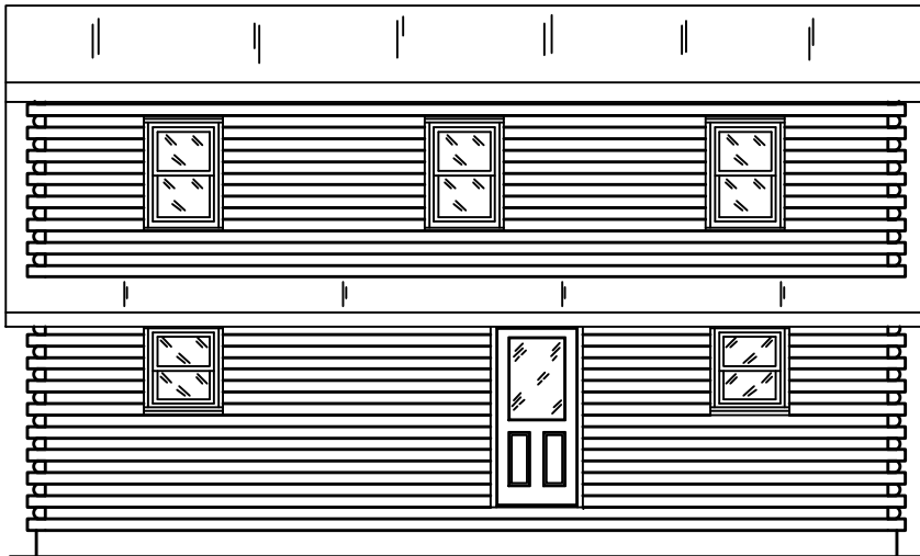
ELEVATION C
