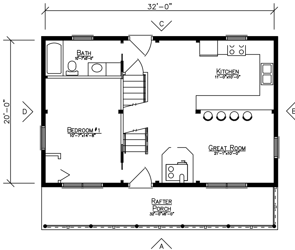
FLOOR PLAN
